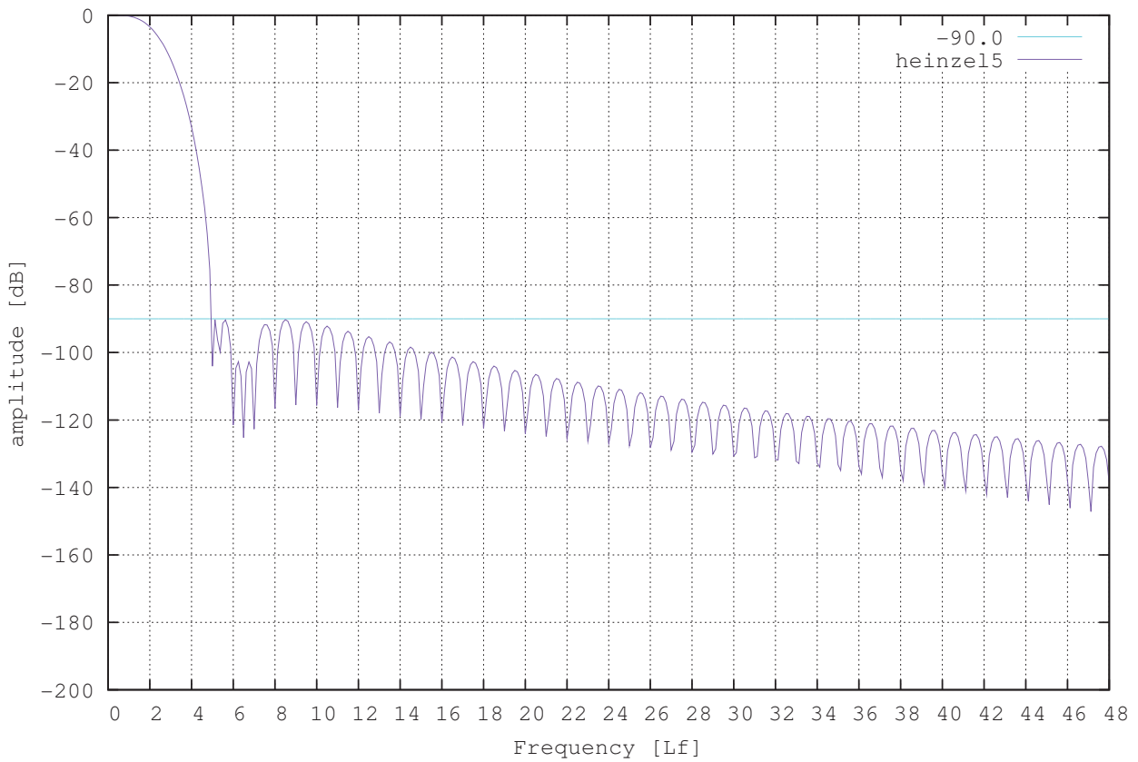
DFT spectrum of the window function
